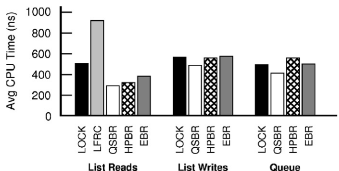
Fig. 6. Base costs—single-threaded data from 8-CPU machine. Y-axis shows Avg CPU time , defined as the average per-operation execution time multiplied by the number of threads.
